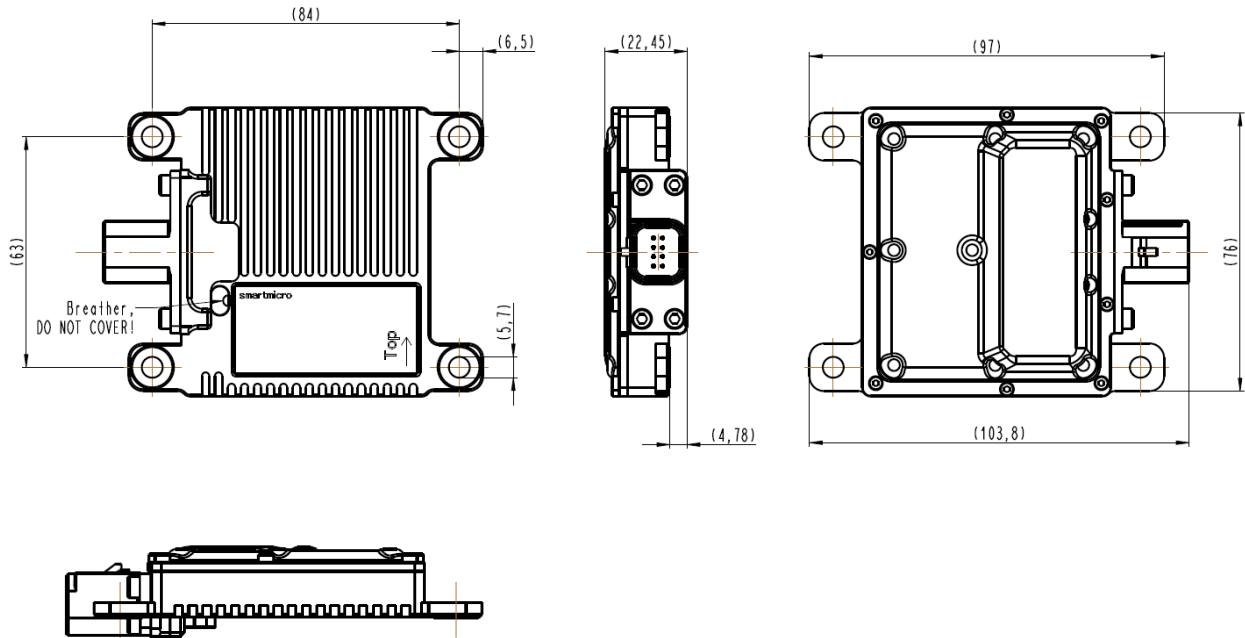
Figure 8: Sensor Dimensions
