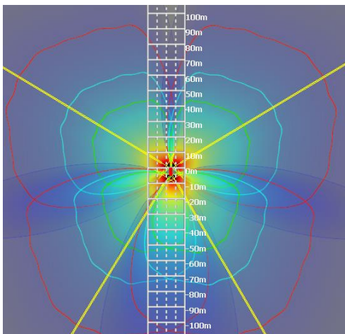
Figure 4: Four sensors configuration and 360^\circ field of view by using straight antennas.
