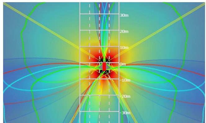
Figure 4: Four sensors configuration and 360^\circ field of view by using straight antennas.
