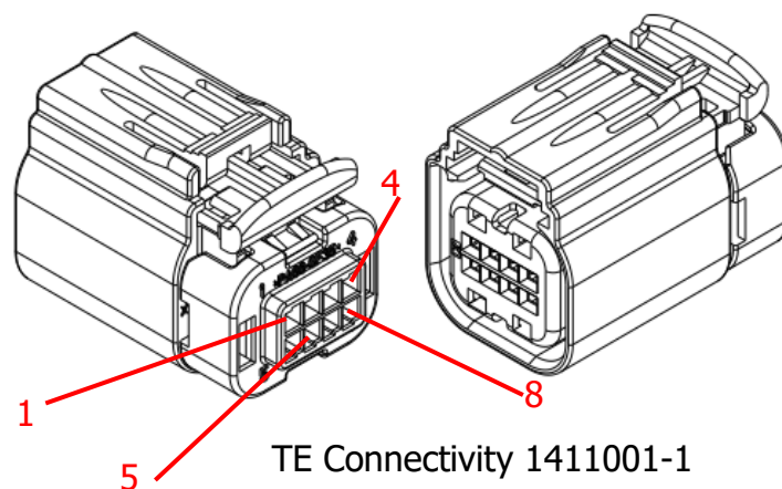
Figure 9: Diagram of cable-FF025 and rear view of female counterpart
